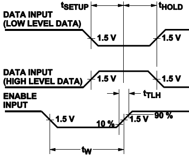
Figure 1. Timing Diagram of 5082-7300 Series Logic.
