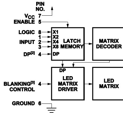
Figure 2. Block Diagram of 5082-7300 Series Logic.
